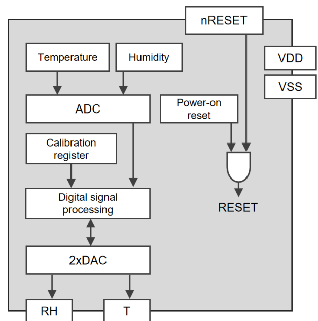
Figure 2. Functional block diagram of GXHT31A
