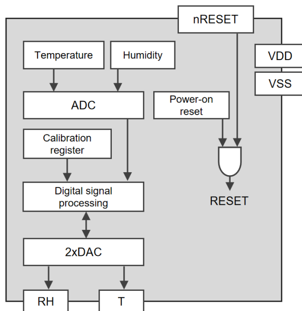
Figure 2. Functional block diagram of GXHT30A
