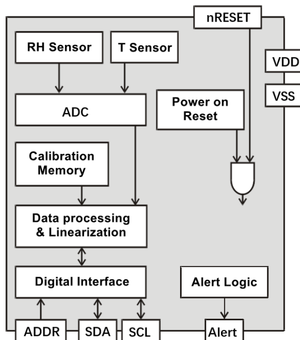
Figure 2. Functional block diagram of GXHT30
